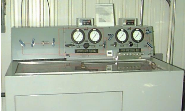
Figure 2.3.1 Burst Test Equipment
