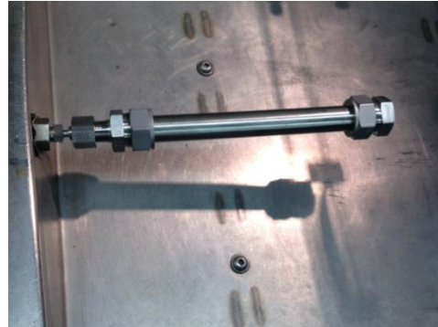
Figure 2.3.2 Burst Test Configuration
