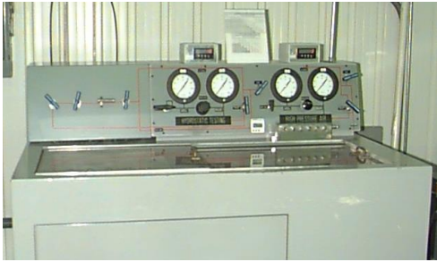
Figure 2.2.1 Gas Leak Test Equipment
