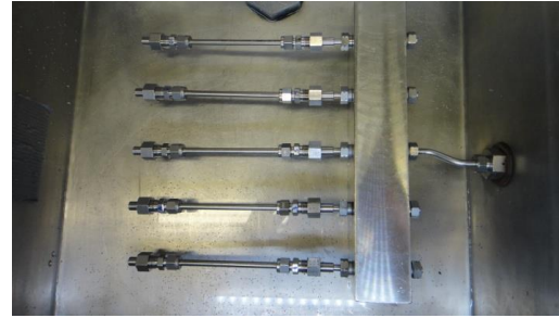
Figure 2.2.2 Gas Leak Test Configuration
